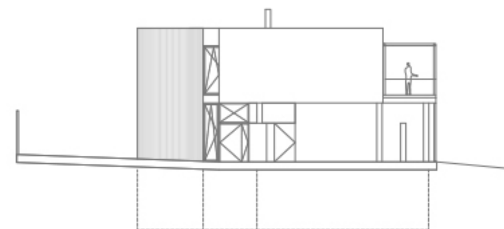
Alzado Norte/ North Elevation
